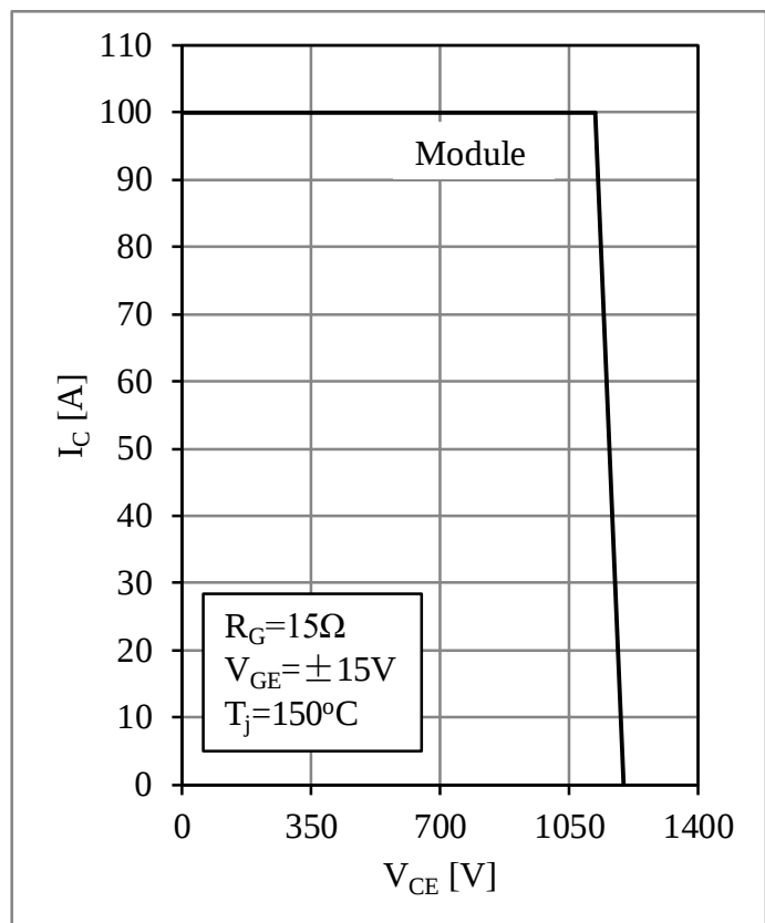
Fig 5. IGBT-inverter RBSOA
