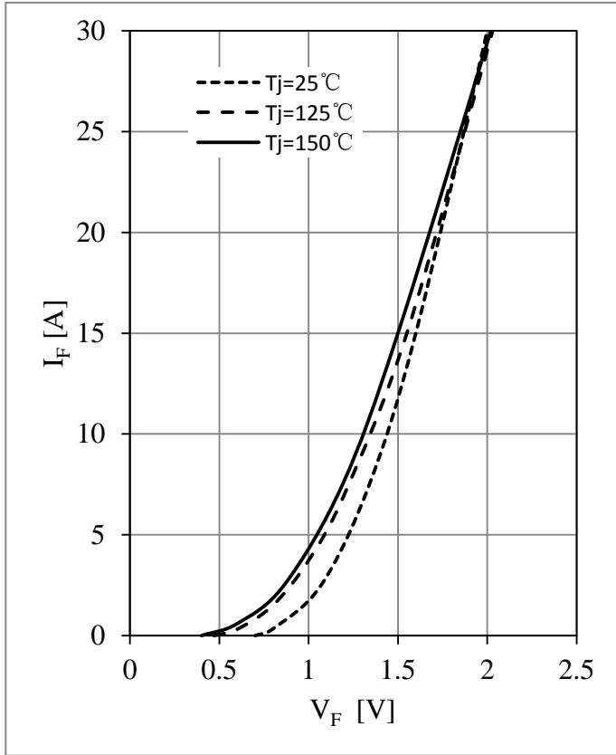
Fig 13. IGBT-brake Output Characteristics
